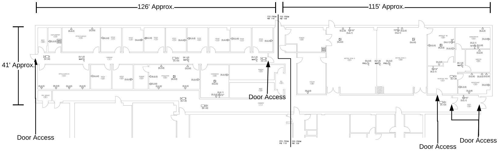
Cable Drop Detail - Main Level SCALE: 1/8" = 1'
